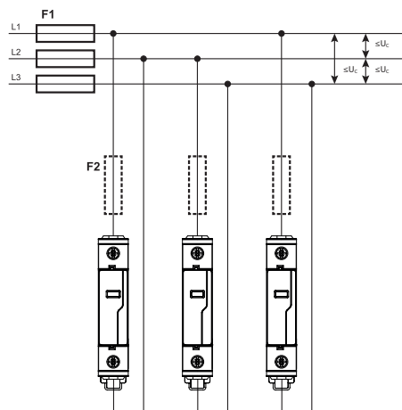
TN, TT, IT
