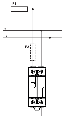
TN-S, TT (1+1)
