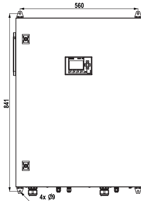
Fig. 4: Mounting holes
