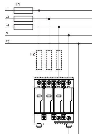
TN-S, TT (3+1)
