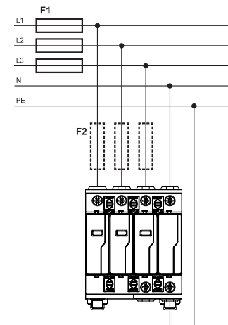
TN-S, TT (3+1)
