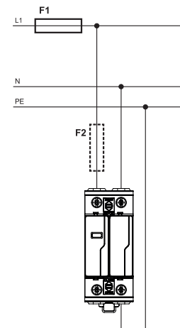
TN-S, TT (1+1)
