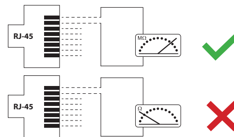
Svorky pro test / Terminals for test
