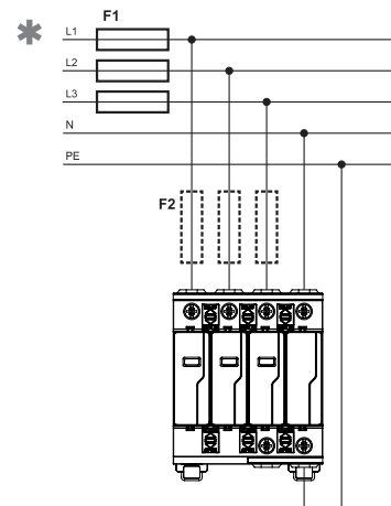
TN-S, TT (3+1)
